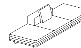
3 seats Variant 2 Size: W3300xD1100xH675 xHS415 mm
