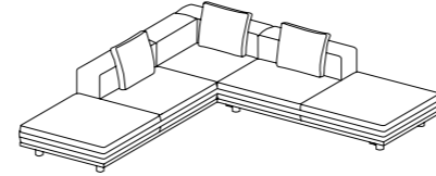
Corner Variant 3 Size: W3300xD3300xH675 xHS415mm
